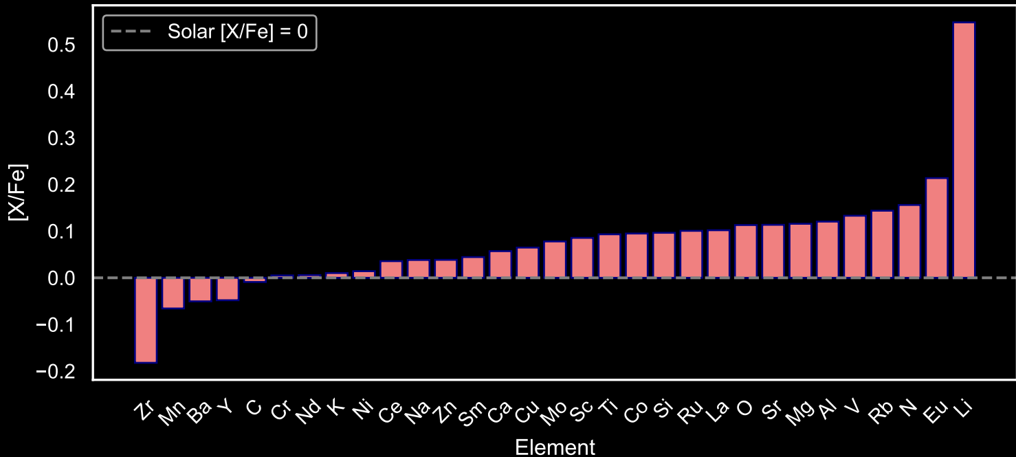
Abundance Pattern for GALAH Star Field [21] (N=275)
