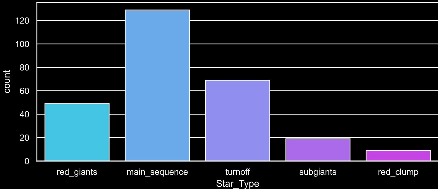
Field [21] Count plot of Star Type
