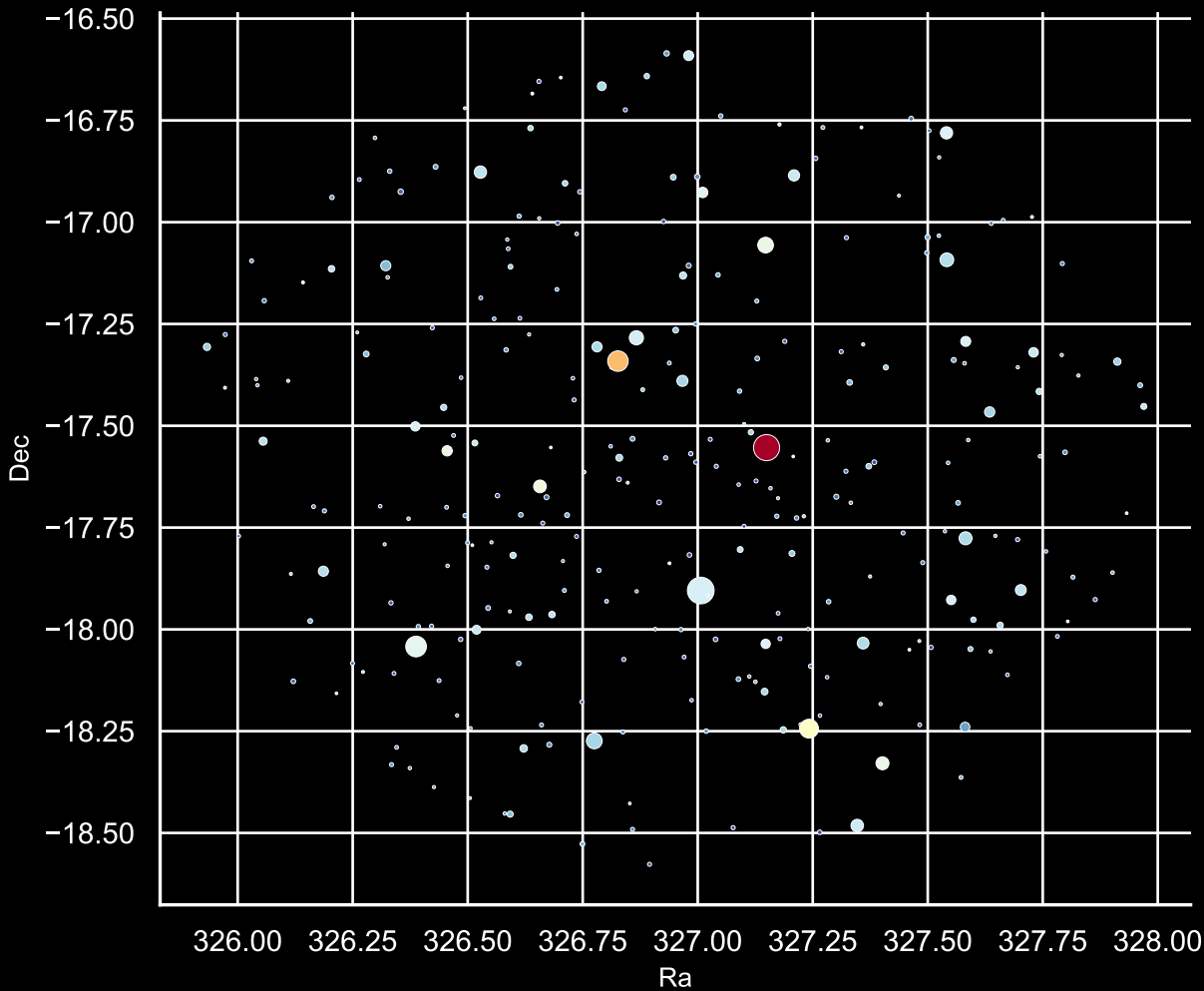
Field [21] Ra [326.94] Dec [-17.6] Stars: 275
