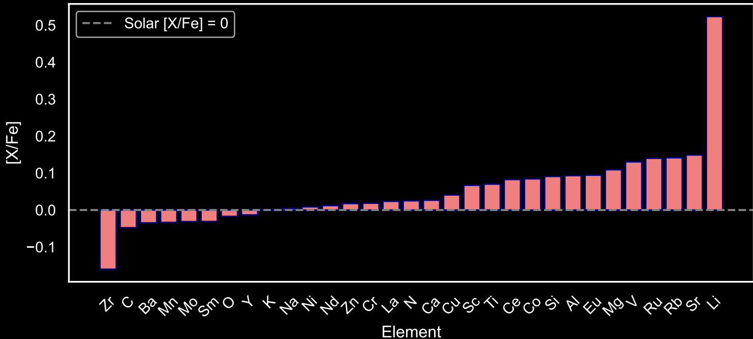
Abundance Pattern for GALAH Main Sequence Stars: Star Field [21] (N=129)
