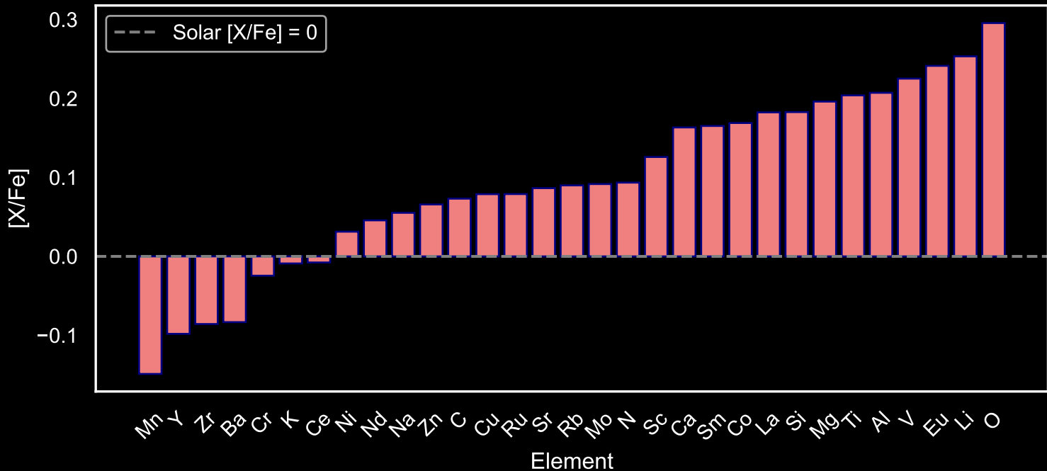
Abundance Pattern for GALAH Red Giants: Star Field [21] (N=58)
