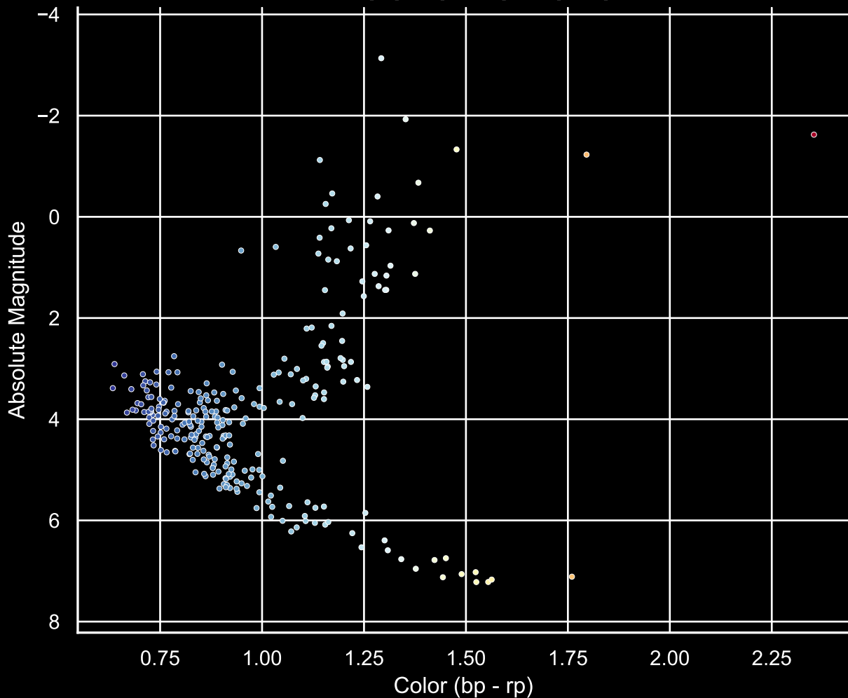
GALAH Hertzsprung-Russell Diagram Field [21] Ra [326.94] Dec [-17.6]
